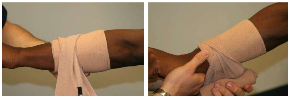
Figure 2-2 Pressure Bandage
